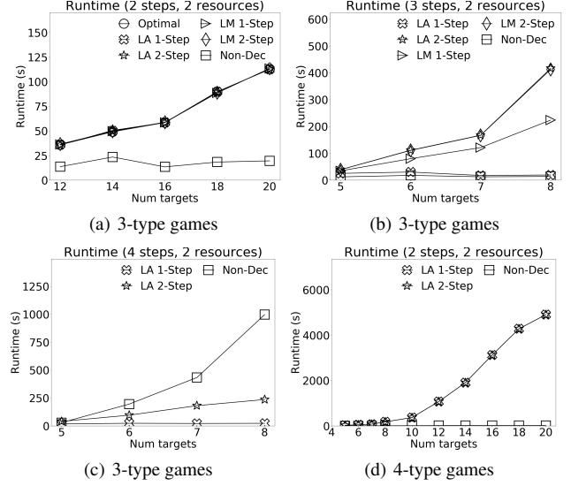
Figure 4: Runtime performance
